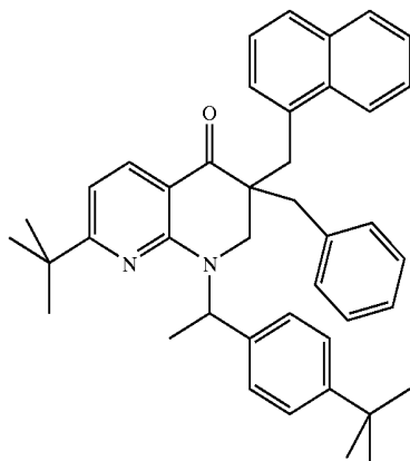
Chemical Formula 2-j
