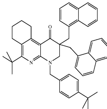
Chemical Formula 2-n
